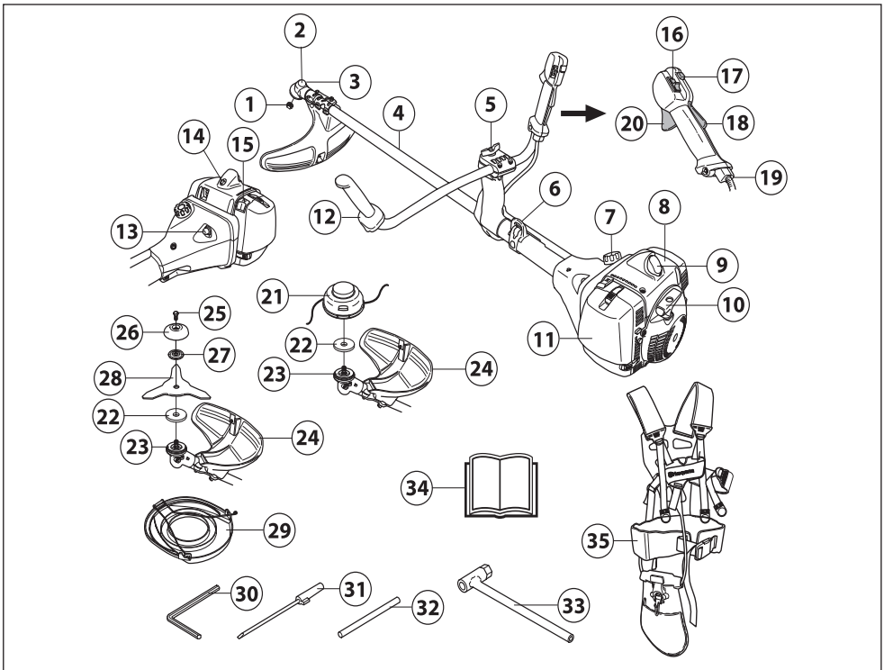
What is what on the brush cutter? (555RXT)
